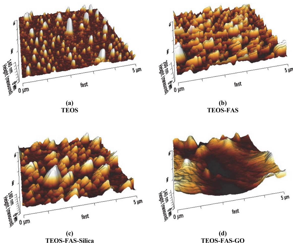
Fig. 4: Atomic force microscopy for different hydrophobic coating surfaces (a) TEOS sol, (b) TEOS-FAS, (c) TEOS-FAS-Silica and (d) TEOS-FAS-GO
