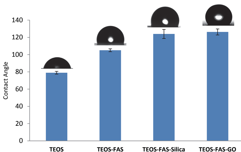
Fig. 1: Contact angle for different hydrophobic coating surfaces
