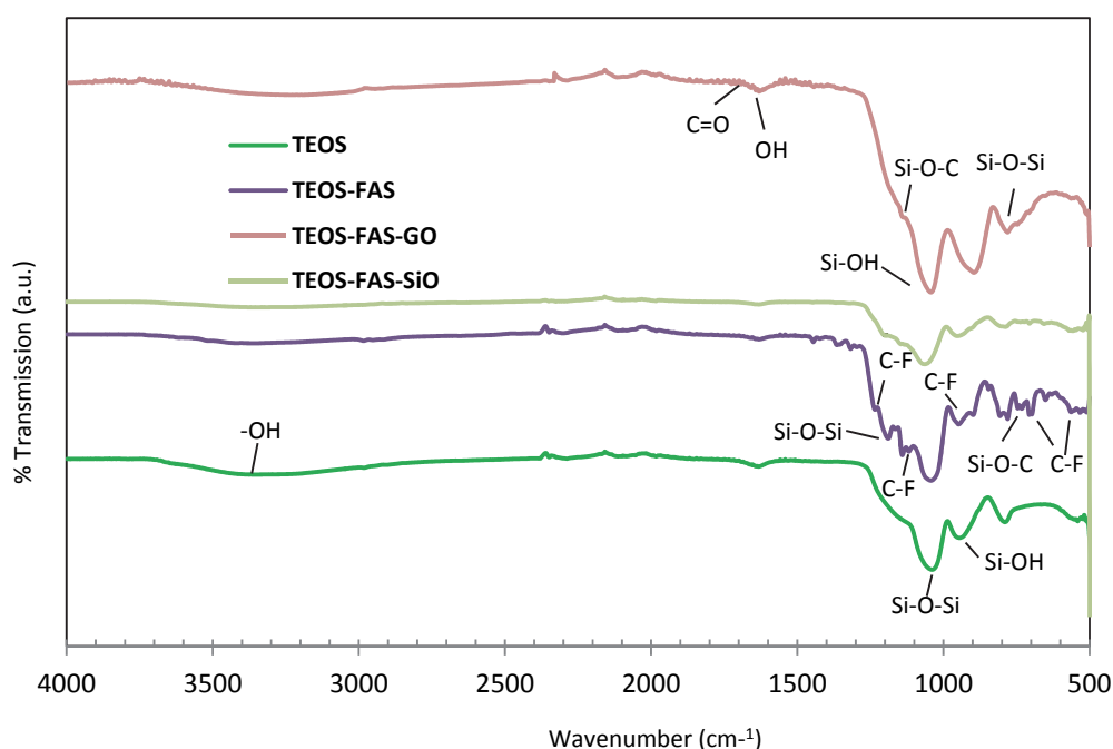
Fig. 3: FTIR spectra for different hydrophobic coating surfaces
