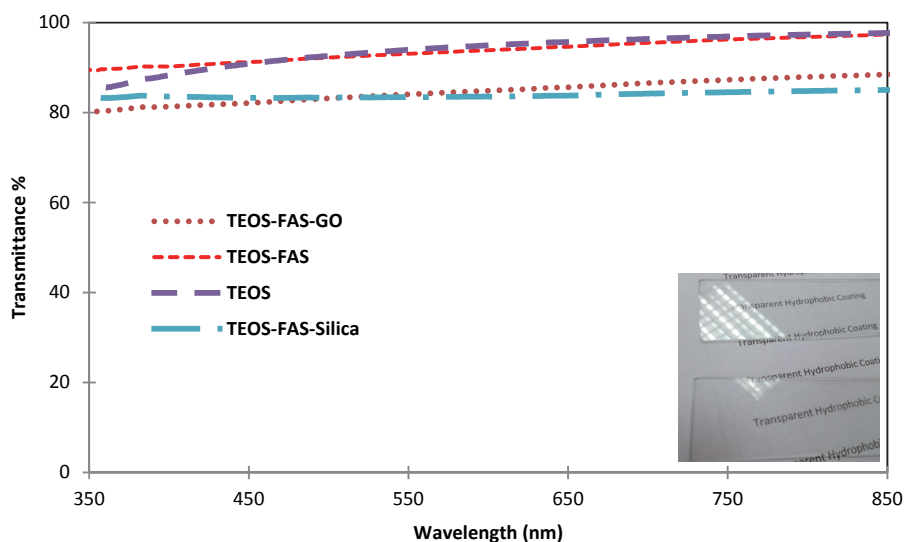
Fig. 2: UV-Visible spectra for different hydrophobic coating surfaces. The inset photo shows the transparency of hydrophobic coating micro slides
