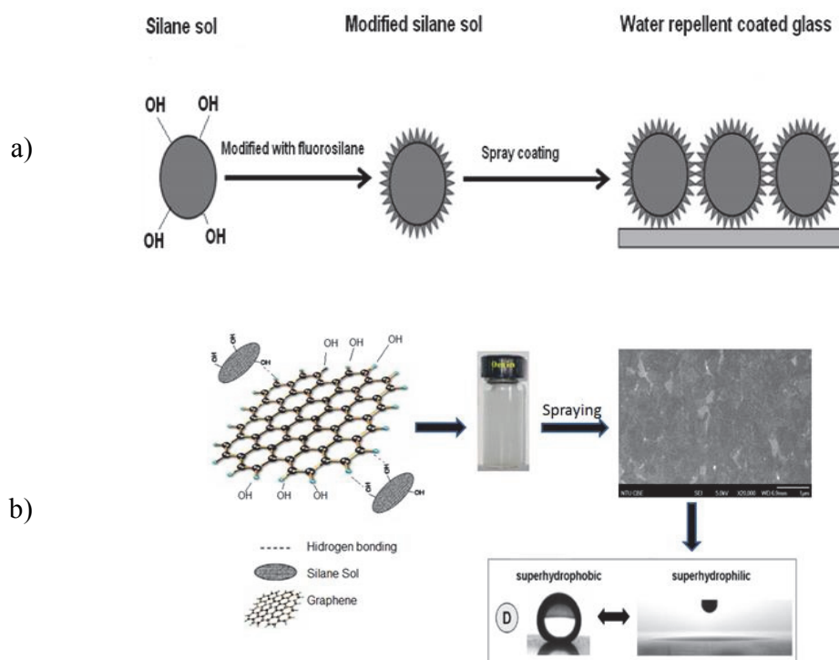
Scheme 1: Schematic formulation of hydrophobic coating using (a) silica and (b) GO by sol-gel method
