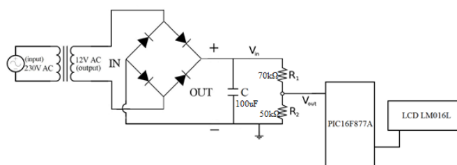
Figure 10. Circuit schematic of the digital voltmeter.
