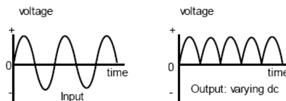
Figure 7. Sinusoidal waveform is converted to half wave [4].
