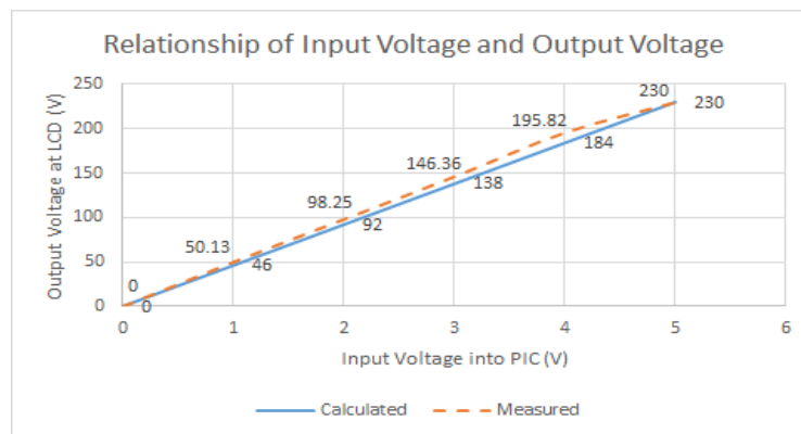
Figure 11. Relationship of input voltage and output voltage.
