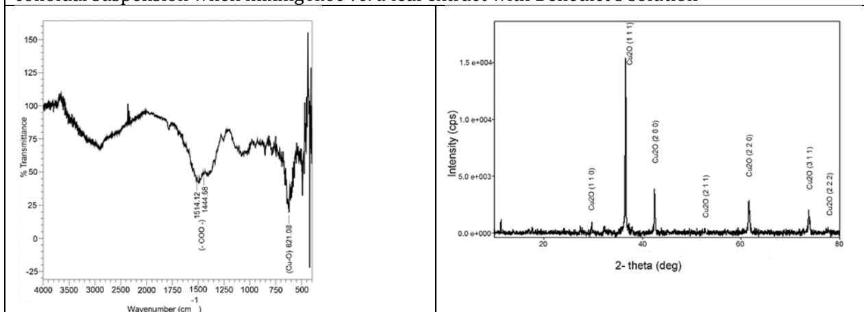
FIGURE 5. FTIR spectra of green synthesized cuprous oxide nanoparticles in green color colloidal suspension when mixing Aloe vera leaf
