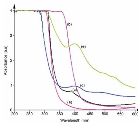
FIGURE 1. UV-VIS spectra for (a) Benedict's solution, (b) Aloe vera extract, (c) colloidal suspension after converted to Green color, (d) colloidal suspension after converted to yellow brown color and (e) colloidal suspension after converted to brick red color.
