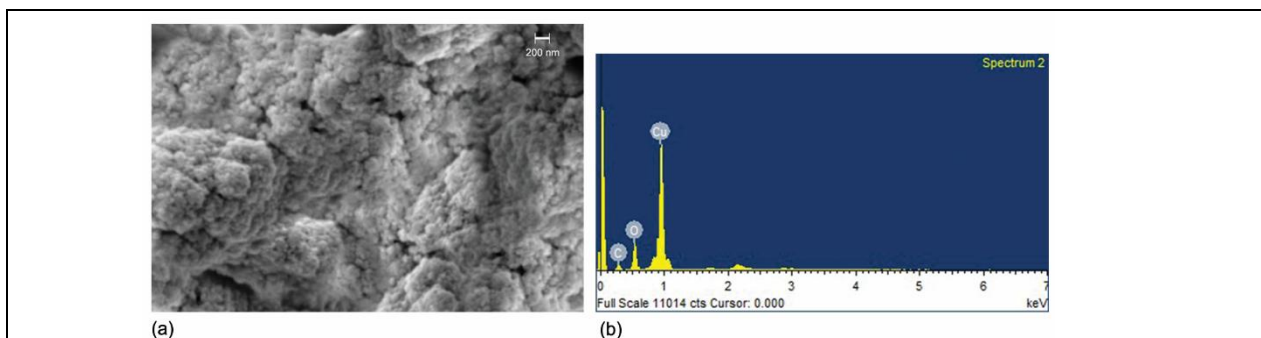
FIGURE 4. (a) SEM image (b) EDX Profile taken from the cuprous oxide particles in green color colloidal suspension when mixing Aloe vera leaf extract with Benedict's solution
