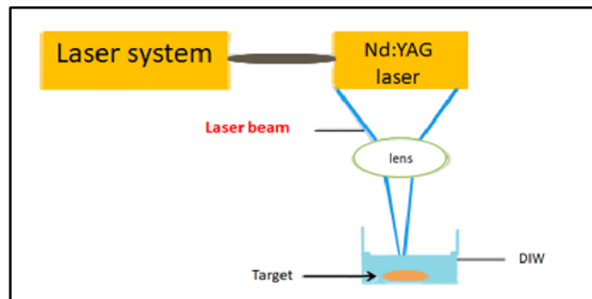
Fig. 1: The essential features of Nd-YAG laser.
