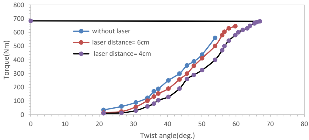
Fig. 3: Torque force as a function of twist angle of 8 minutes exposure time with and without laser treatment
