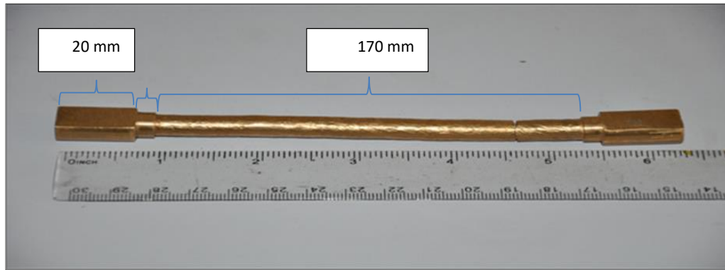
Fig. 2: Metal Sample after torsion testing
