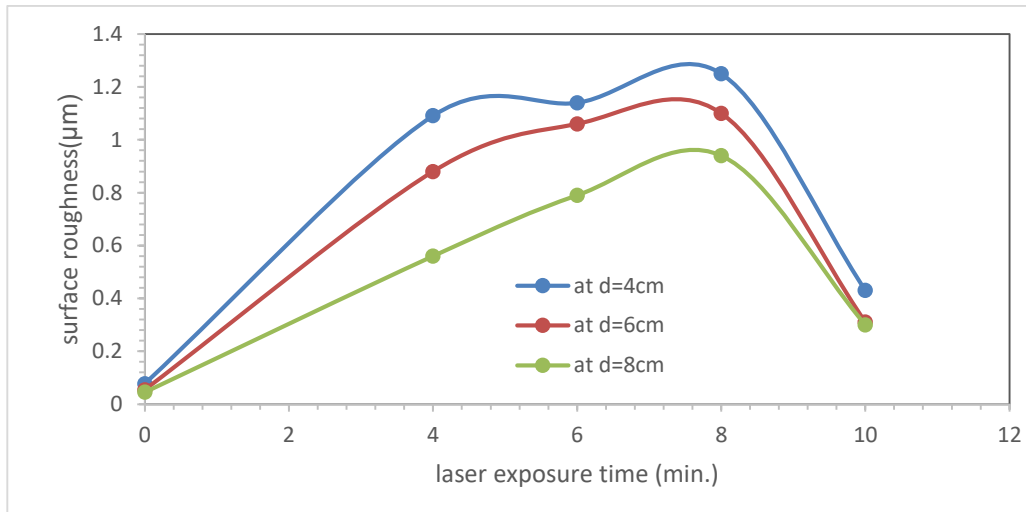
Fig. 5: Surface roughness versus laser exposure time for 4 cm, 6cm and 8 cm distances from laser source.
