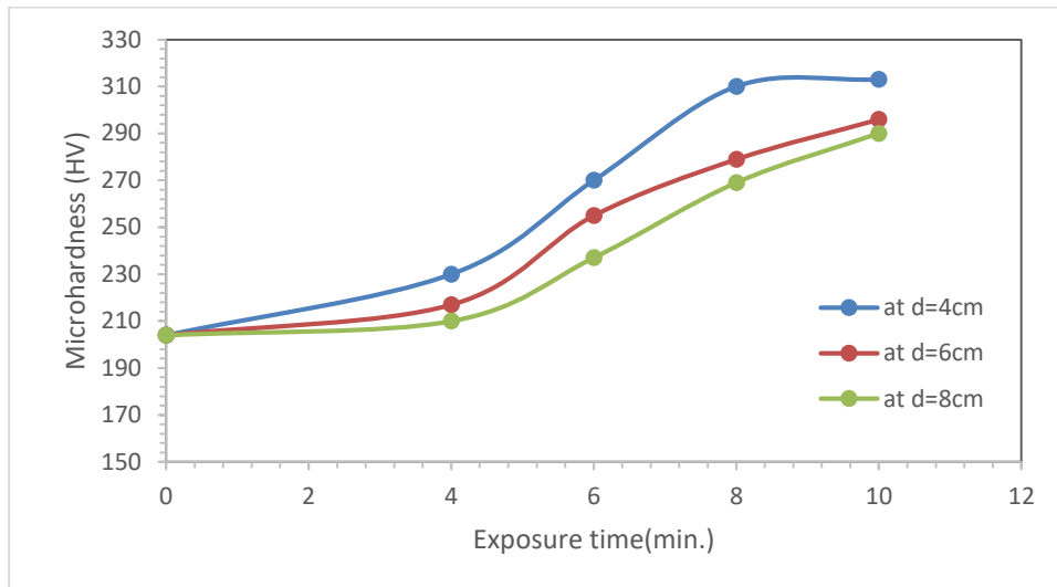
Fig. 6: Micro hardness versus laser exposure time of 4 cm, 6 cm and 8 cm of distance from laser source
