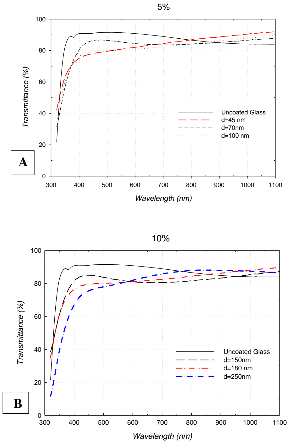
Fig.(8)Effect of ITO thickness variation on the transmission of glass vs. wavelength for different concentration (A) 5% , (B) 10%.
