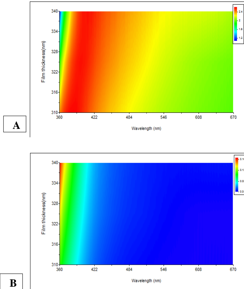
Fig.(7) Contour lines of : (A) n - and (B) k - values due to thickness and wavelength variation.
