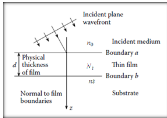
Fig.(1) Plane waves incident on thin- film[27]
