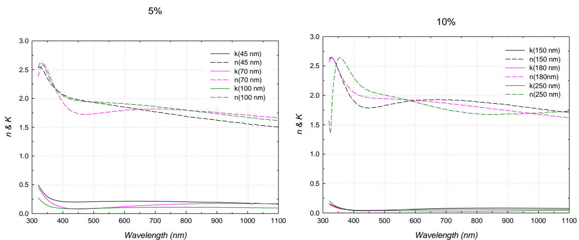
Fig. (6) The effect of ITO thickness on the refractive index and extinction coefficient of film vs. wavelength for impurity ratios 5% and 10%.
