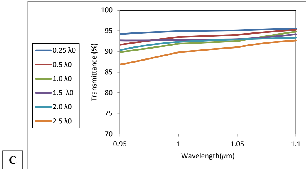
Fig.(5) Computed transmittance of ITO /Glass at different design wavelength: (A) \lambda_0=0.550 \text{ nm} , (B) \lambda_0=0.6328 \text{ nm} and (C) \lambda_0=1.064 \text{ }\mu\text{m} .
