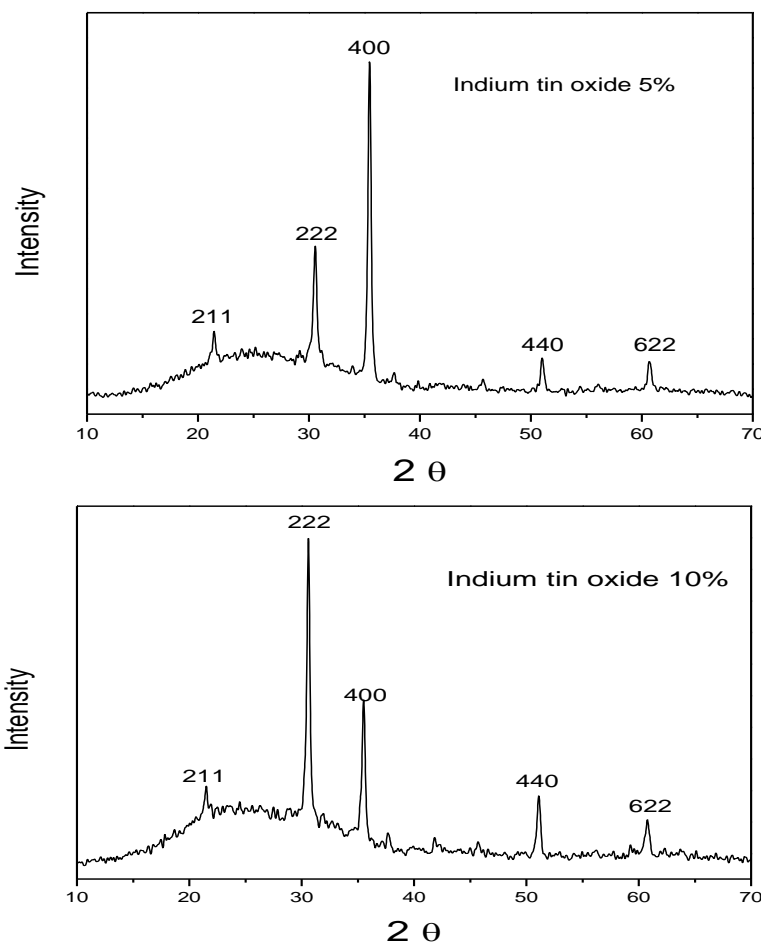
Fig. 2 XRD patterns for indium tin oxide a) 5% Sn concentration b) 10% Sn concentration.
