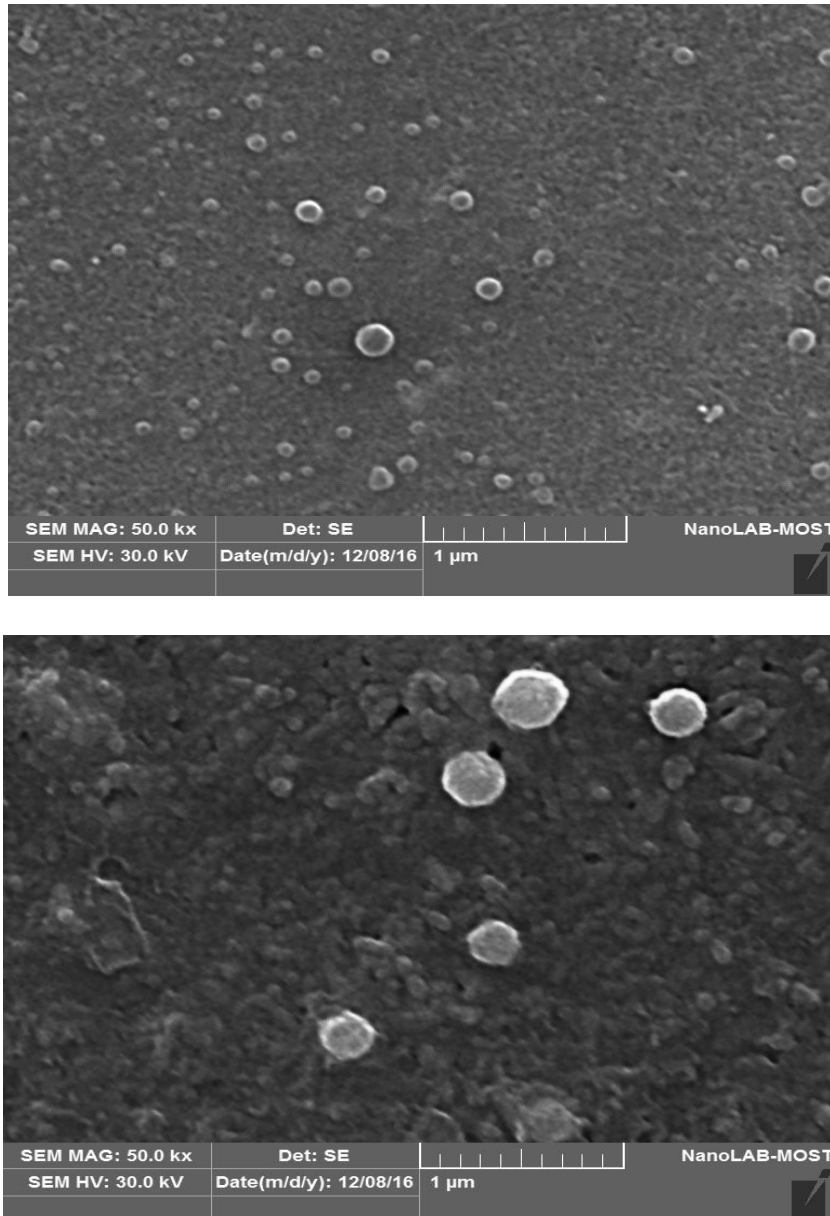
Fig. 4 SEM images of indium tin oxide a) 5% Sn concentration b)10% Sn concentration
