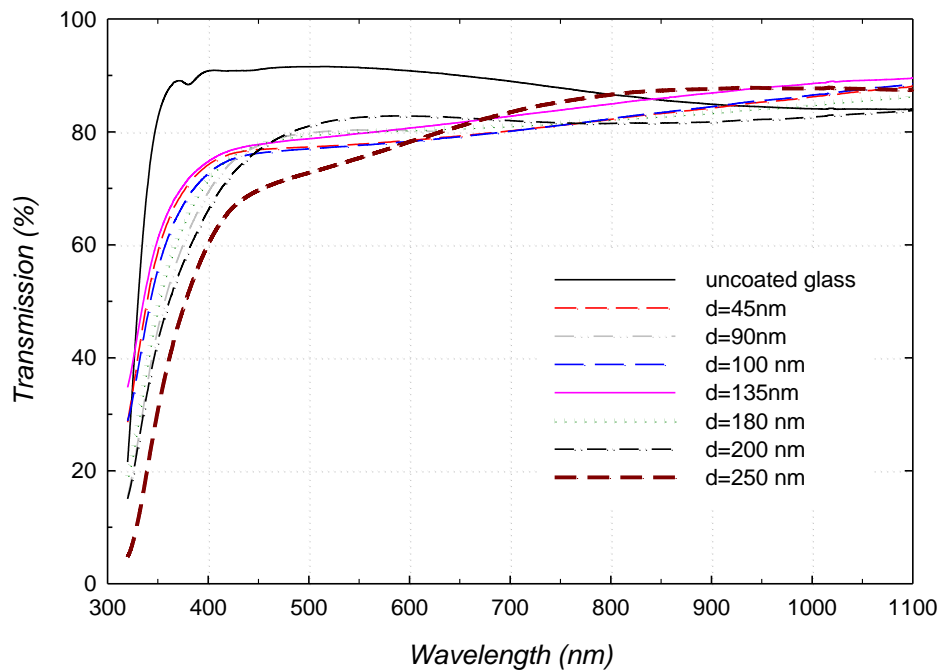
Fig.(9) Measured transmission of ITO / glass vs. wavelength of 5% concentration over thickness range (45-250 nm).
