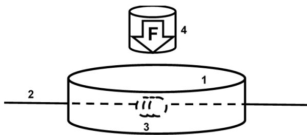
Figure 1. Fibre coil sandwiched rubber subjected to a load F : (1) rubber rod; (2) optical fibre; (3) fibre coil; and (4) load F .
