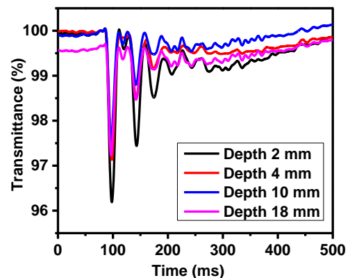
Figure 10. The change in light coming out of the fibre describing stress history as the rubber was subjected to the impact loading of 4 kg.
