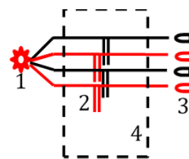
Figure 4. Basic experimental setup for measuring transient response time at four different points inside the rubber: (1) light source, (2) closely arranged fibre coils, (3) light detectors, (4) rubber bar.
