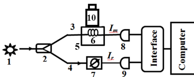
Figure 3. Experimental setup used to measure transient response time. (1) light source, (2) splitter, (3) modulated optical fiber, (4) reference fiber, (5) silicone rubber, (6) fiber sensor, (7) attenuator, (8) photo-detector #1 and (9) photo-detector #2 and (10) load
