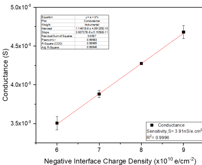
Figure 14. The conductance of silicon nanowire biosensor according with different concentration of interface charge density, Q_F .
