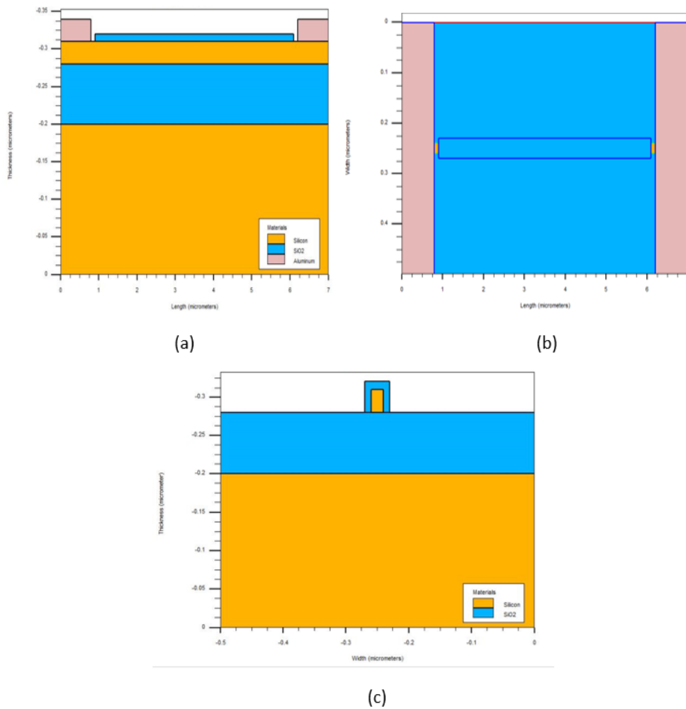
Figure 11. Simulated model of silicon nanowire biosensor in 2D views with cross-sectional along (a) x-axis, (b) z-axis and (c) y-axis.
