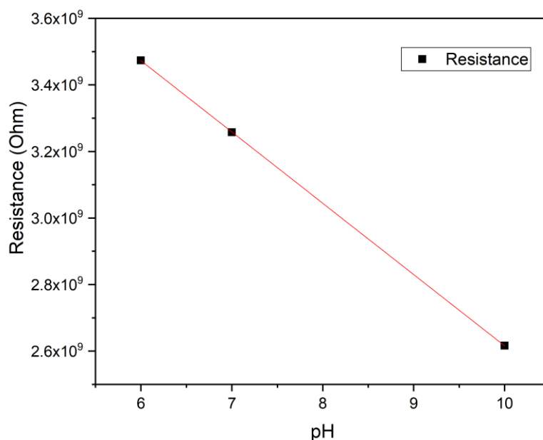
Figure 8. Average resistance value of silicon nanowire pH sensor according to pH level detection.
