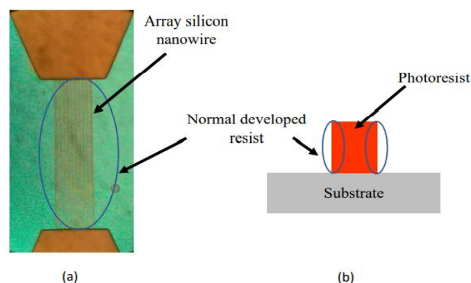
Figure 3. The normal developed or desired pattern structure of (a) array nanowire and (b) cross section view.
