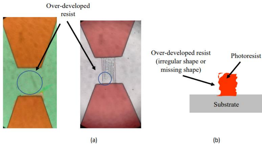
Figure 5. The over-developed resist of (a) array nanowire and (b) cross section view.
