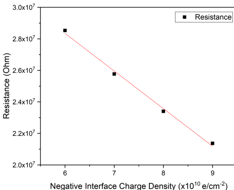
Figure 13. The resistance of simulated silicon nanowire biosensor according with different concentration of interface charge density, Q_F .
