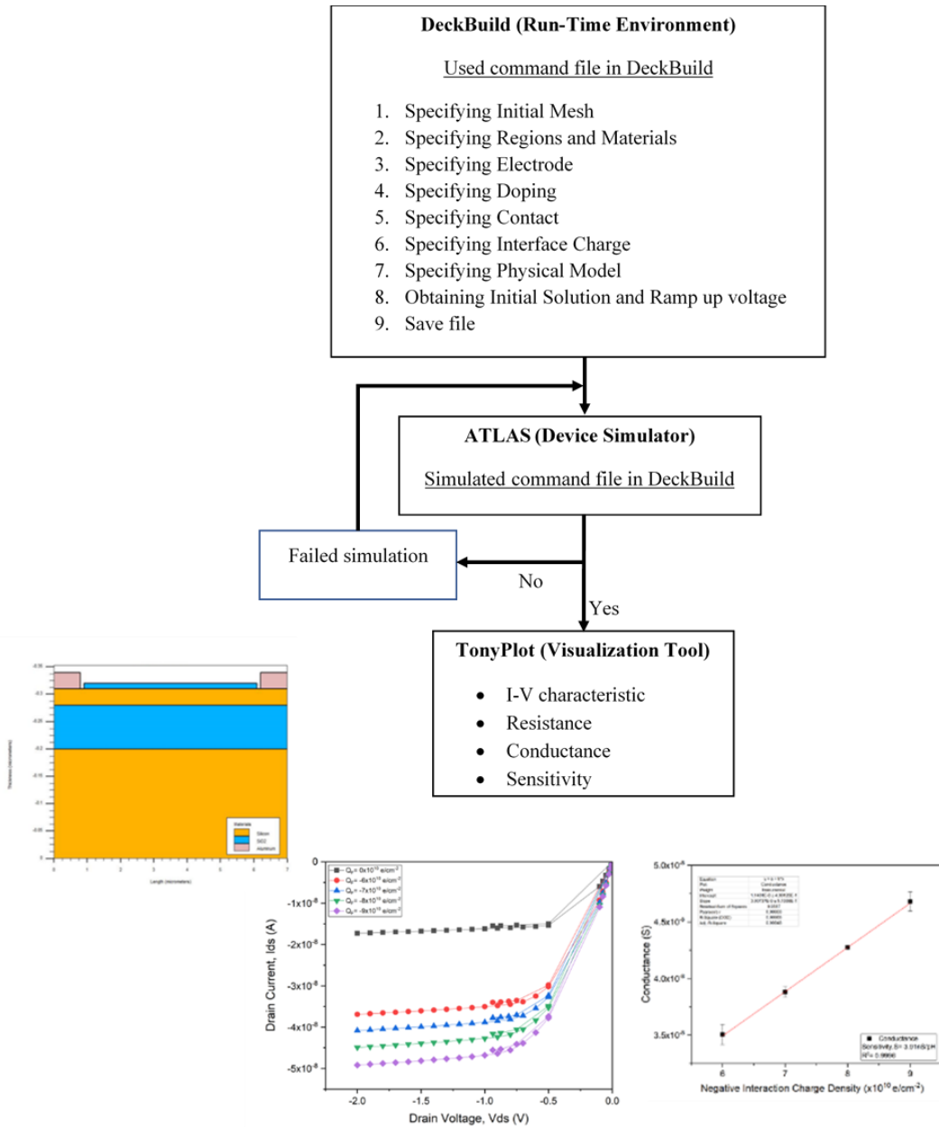
Figure 2. Simulation process of silicon nanowire biosensor.
