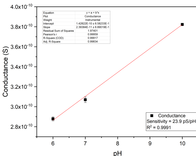
Figure 9. Average conductance value of silicon nanowire pH sensor according to pH level detection.
