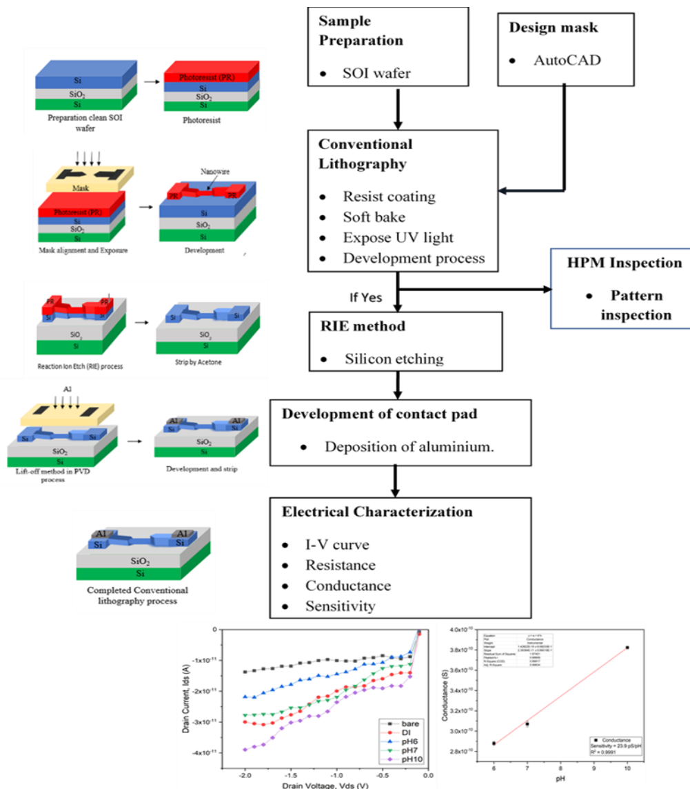
Figure 1. Fabrication process of silicon nanowire pH sensor.
