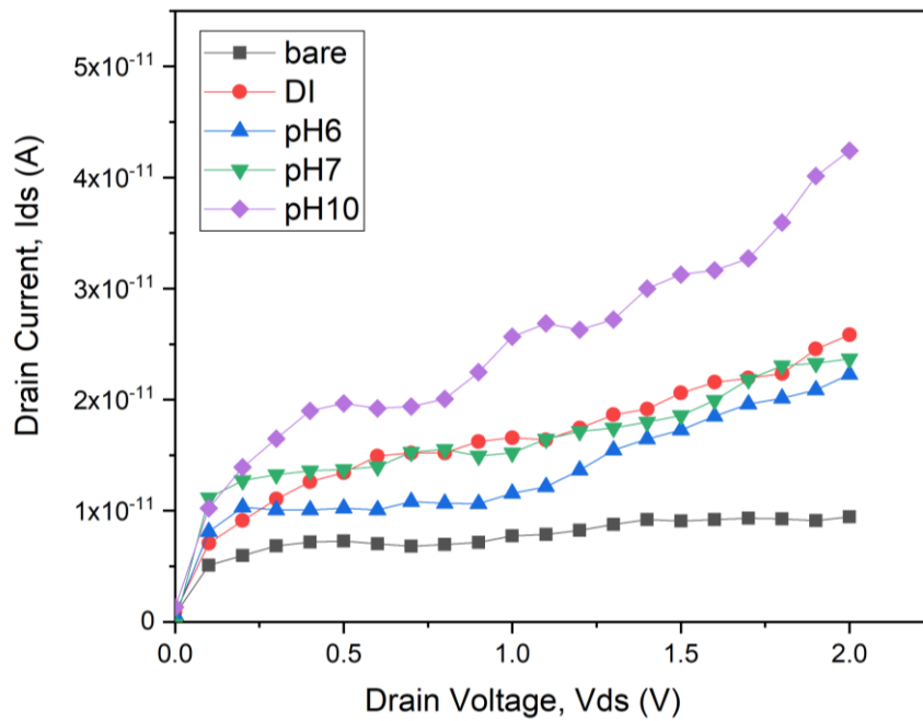
Figure 7. pH level detection of bare, DI water, pH6, pH7 and pH10 with positive voltage.
