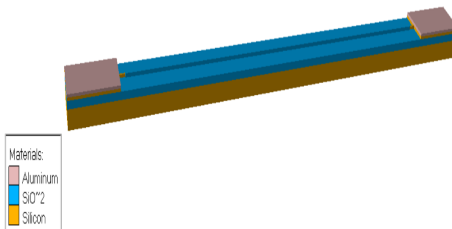
Figure 10. Simulated model of silicon nanowire biosensor in 3D view.
