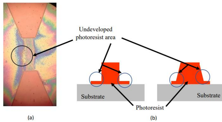
Figure 4. The under-developed resist of (a) array nanowire and (b) cross section view.
