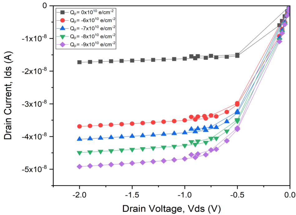
Figure 12. The I-V characteristic of simulated silicon nanowire biosensor according to different concentration of interface charge density, Q_F .
