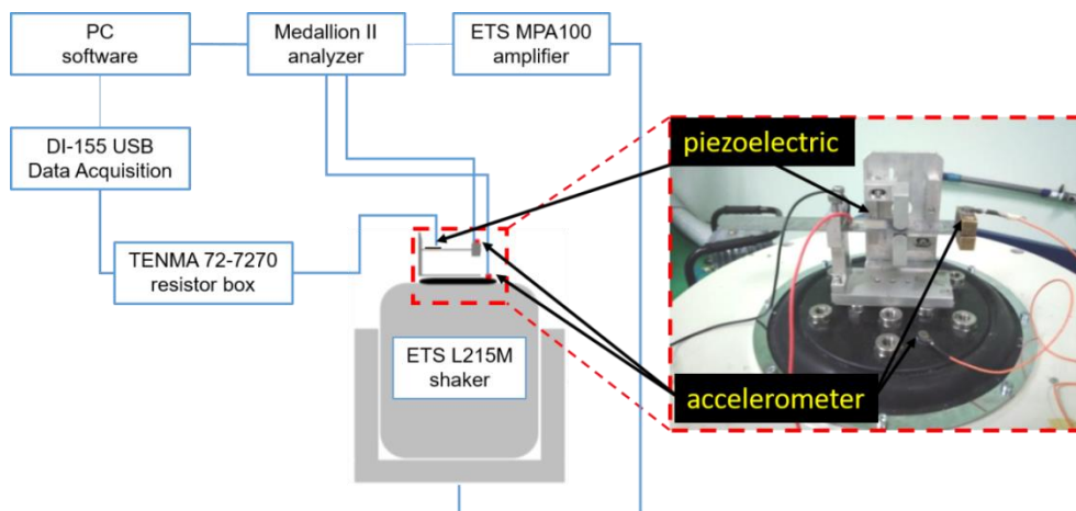
Figure 2. Experimental setup for dynamic measurement
