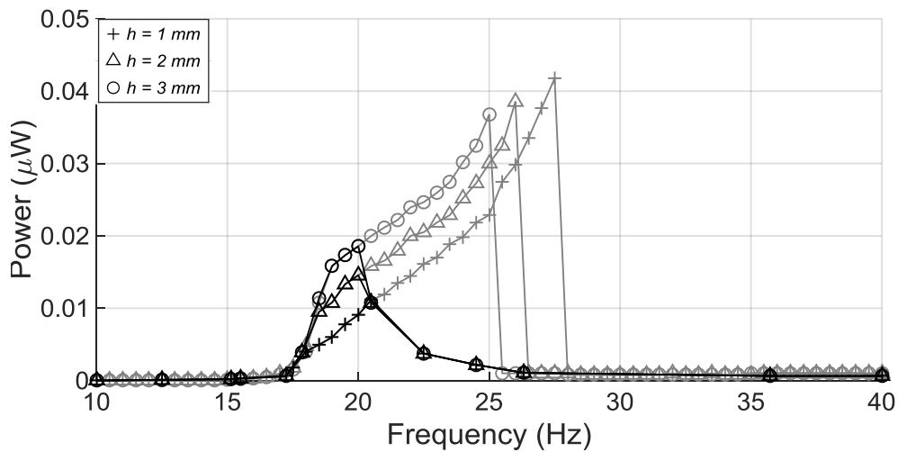
Figure 11. Measured power against frequency for the closed-circuit non-linear system for the different vertical gap, h at b = 45 mm
