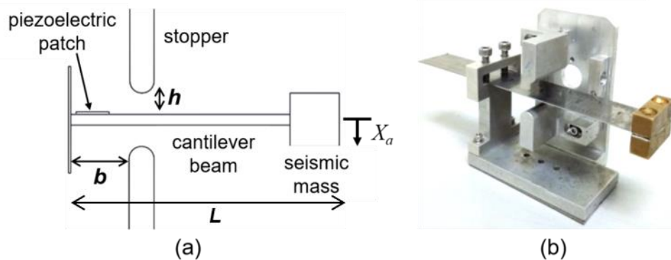
Figure 1. (a) Schematic and (b) photo of non-linear energy harvester
