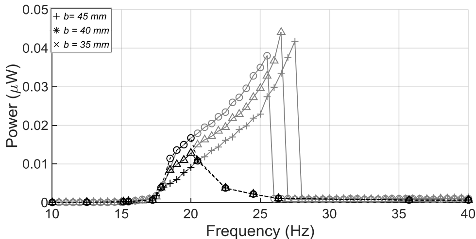
Figure 10. Measured power against frequency for the closed-circuit non-linear system for different horizontal position, b at h = 1 mm
