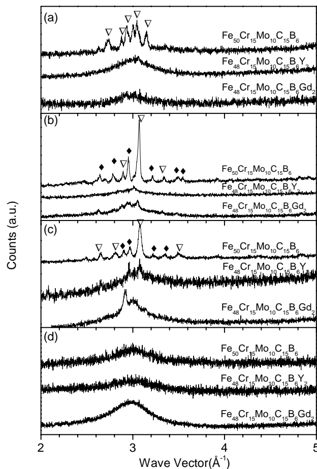
Fig. 1: XRD patterns of (a) down (D), (b) centre (C) and (c) high (H) parts of the wedge and (d) ribbons. Symbols correspond to \text{M}_{23}\text{C}_6 ( \nabla ), \text{M}_6\text{C} ( \blacklozenge ) type carbides.
