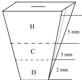
Fig. 2: Wedge shape of the copper mold used for casting, showing the considered parts taken in this study: H (high, 5 mm), C (center, 3 mm) and D (down, 2 mm).
