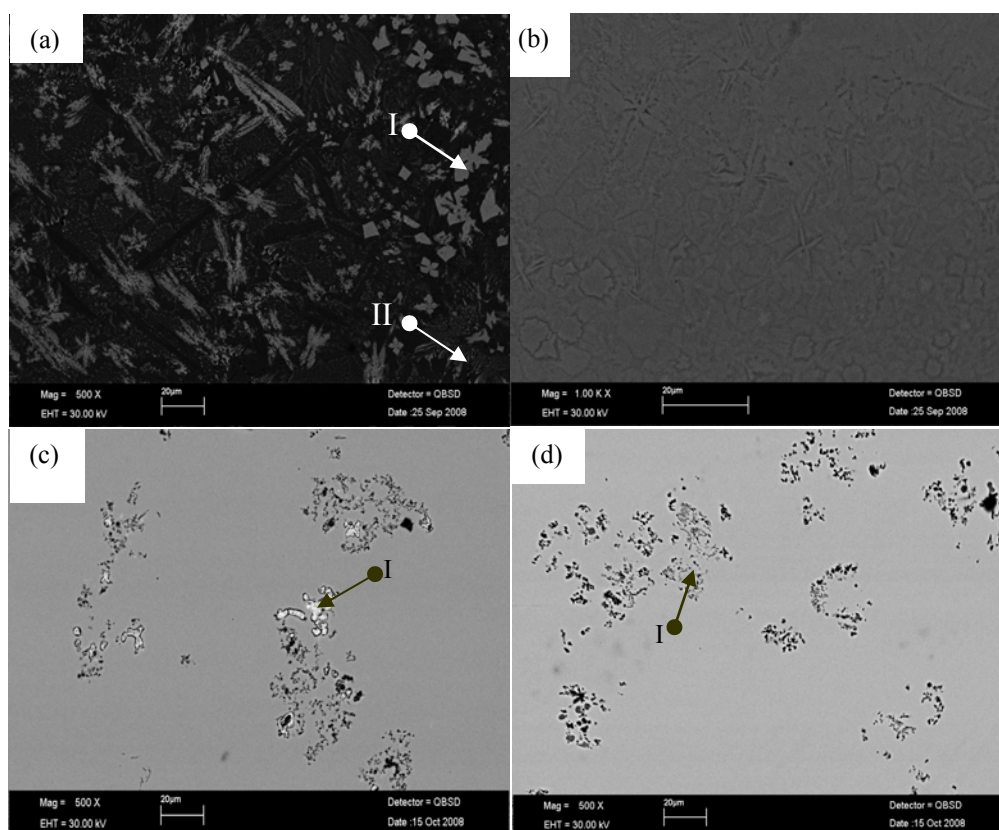
Fig. 3: SEM back scattered electron images of: (a) H part and (b) D part of as-cast \text{Fe}_{50}\text{Cr}_{15}\text{Mo}_{14}\text{C}_{15}\text{B}_6 ; (c) D part of as-cast \text{Fe}_{48}\text{Cr}_{15}\text{Mo}_{14}\text{C}_{15}\text{B}_6\text{Gd}_2 and (d) D part of as-cast \text{Fe}_{48}\text{Cr}_{15}\text{Mo}_{14}\text{C}_{15}\text{B}_6\text{Y}_2 .
