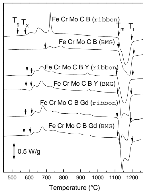
Fig. 4: HT-DSC curves of crystallization and melting for \text{Fe}_{50-x}\text{Cr}_{15}\text{Mo}_{14}\text{C}_{15}\text{B}_6\text{M}_x ( x = 0, 2 and M = \text{Y, Gd} ) as-cast bulk samples (D parts of the wedge) and ribbons.
