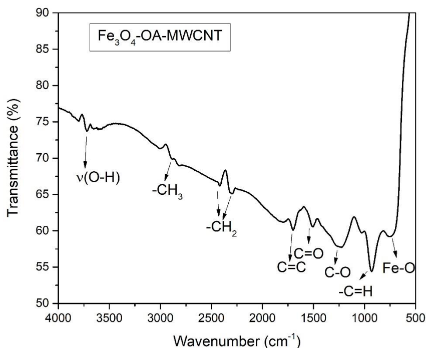
Figure 3: FTIR spectrum of Fe 3 O 4 /OA/MWCNT nanocomposite
