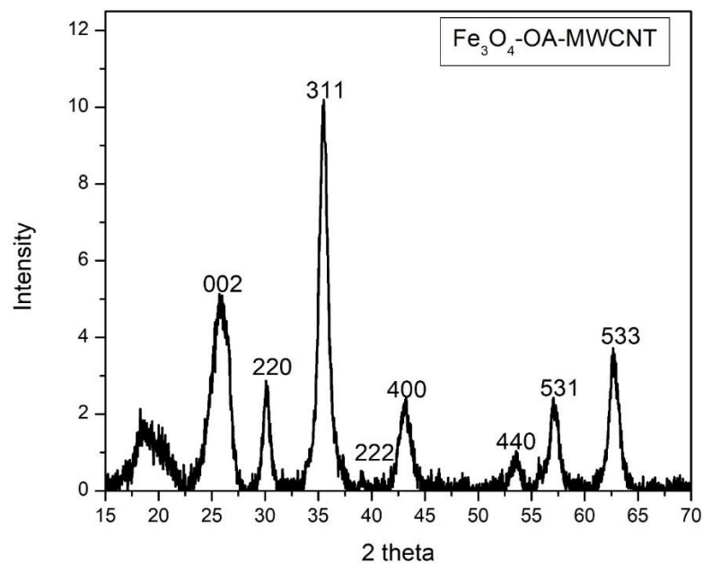
Figure 2: XRD spectrum of \text{Fe}_3\text{O}_4 -OA-MWCNT based nanocomposite
