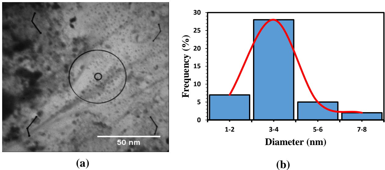
Figure 2. TEM image, size distribution of (a, b) the CdSe QDs synthesized by Pulse Laser Ablation.
