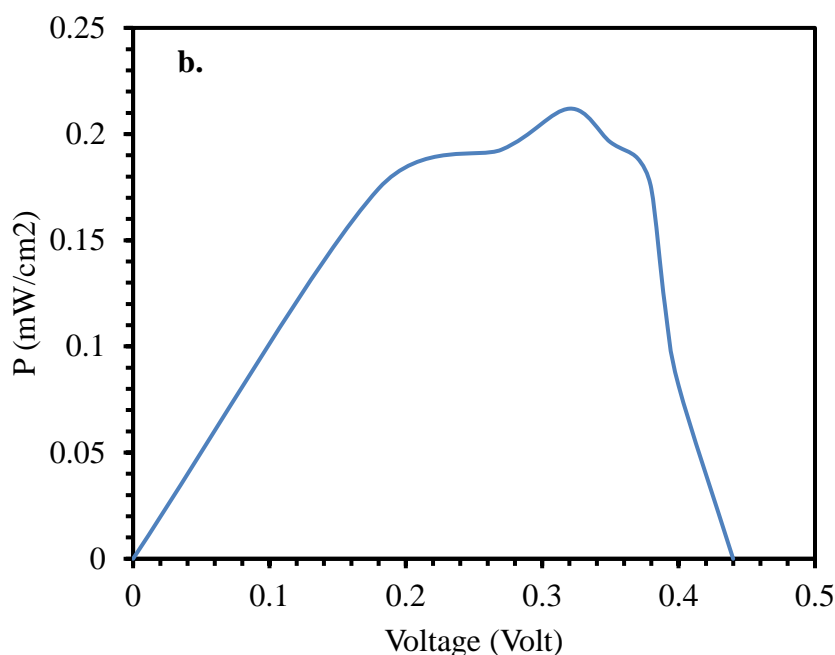
Figure 7. J-V curve for Dye-Sensitized photovoltaic device based CdSe Quantum Dots, (b) the solar cell power response with voltage variation.
