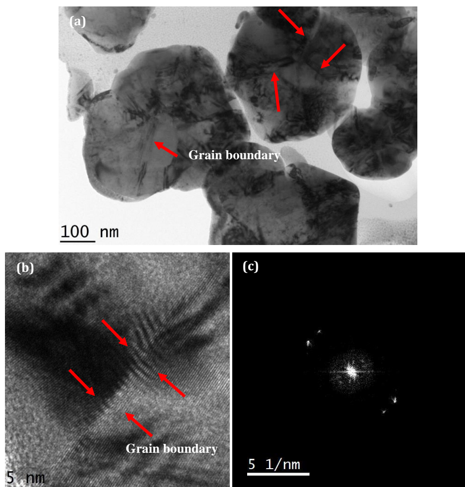
Figure 7. HRTEM micrograph of polycrystalline Ag particle. (a) TEM image, (b) HRTEM image shows the grain boundary and (c) the corresponding FFT pattern.
