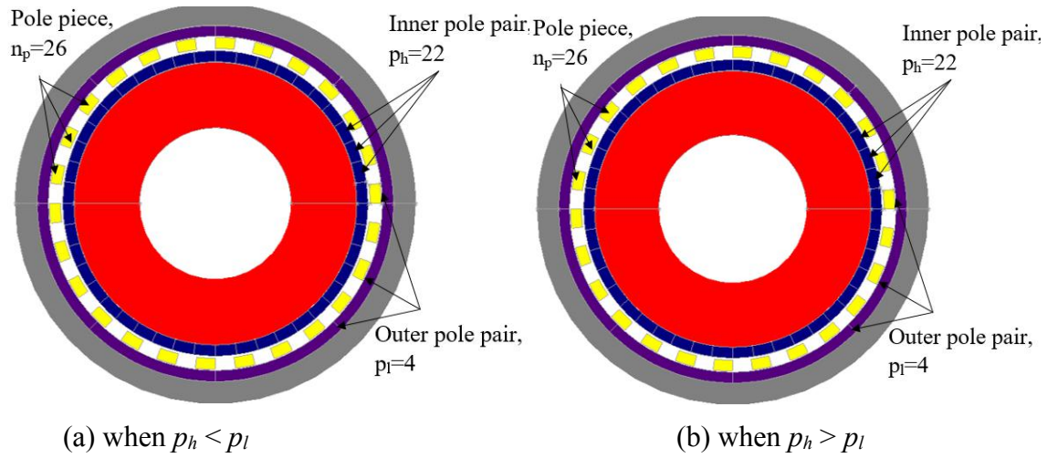
Figure 3. Structure of flux modulation concentric magnetic gear, (a) when p_h < p_l and (b) when p_h > p_l .
