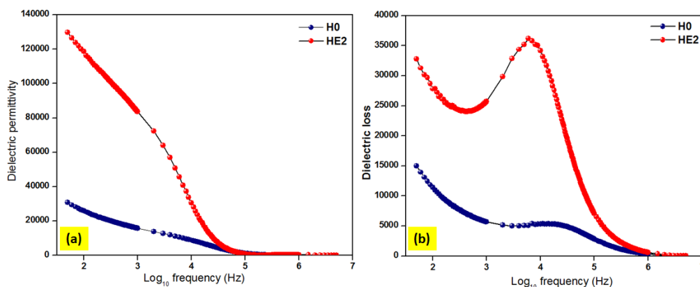
Figure 5. The variation of (a) dielectric permittivity and (b) dielectric loss with logarithm frequency for H0 and HE2 (most conducting SPE).
