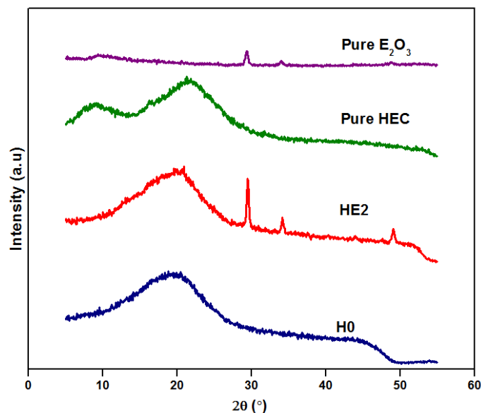
Figure 6. XRD patterns of pure samples (HEC and erbium(III) oxide nanoparticles), H0 and HE2 (most conducting SPE).
