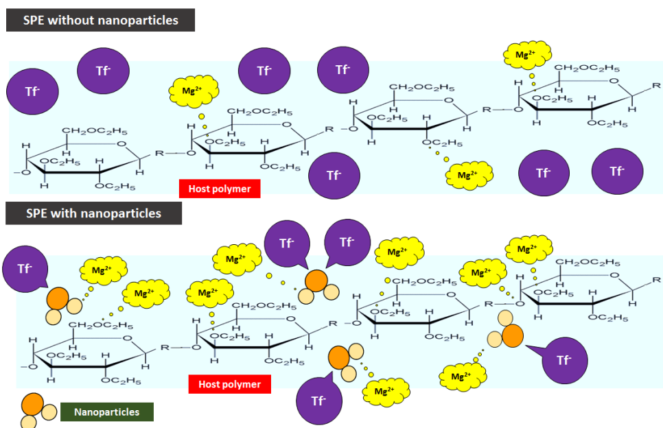
Figure 7. The interactions of the charge carriers in the SPEs (without and with nanoparticles).
