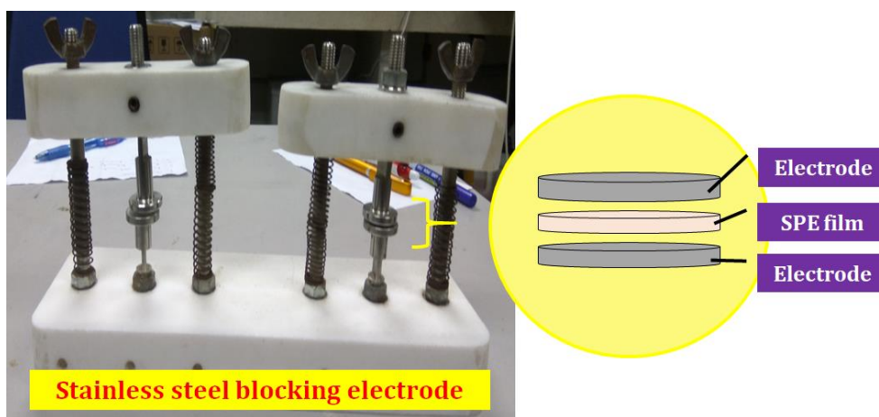
Figure 2. The stainless steel blocking electrode used to sandwich the SPE film for conductivity analysis.
