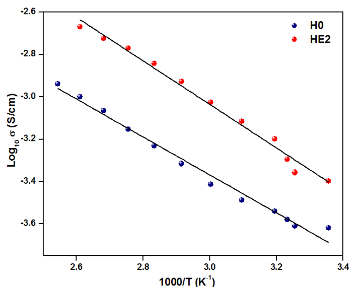
Figure 4. The temperature dependence of ionic conductivities for H0 and HE2 (most conducting SPE).
