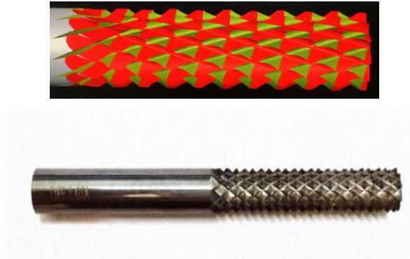
Figure 1. Burr or router tool geometry; CAD model (top); actual tool (bottom).
