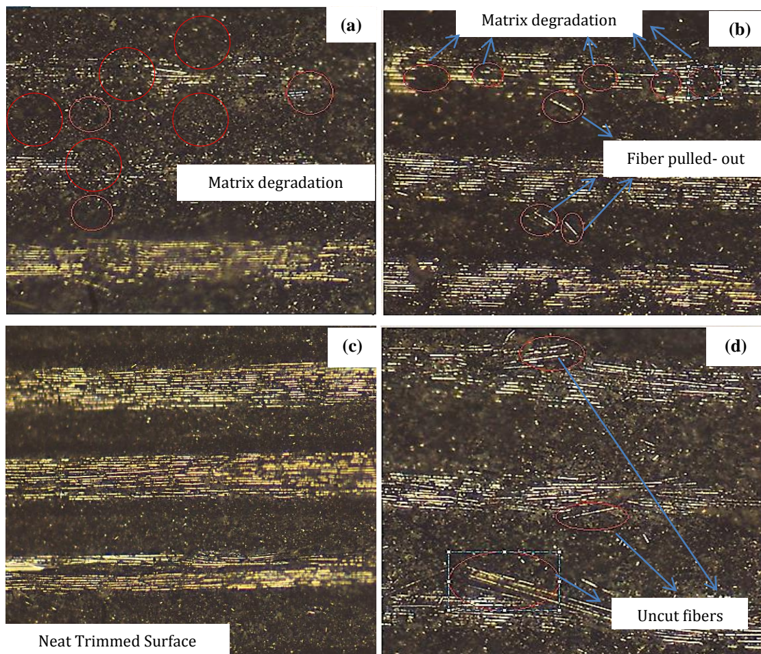
Figure 7. Enlarged of photomicrographs taken on the trimmed surface for various machining conditions; (a) V_c = 100 m/min, f_z = 0.15 mm (b) V_c = 50 m/min, f_z = 0.10 mm (c) V_c = 50 m/min, f_z = 0.15 mm (d) V_c = 150 m/min, f_z = 0.15 mm
