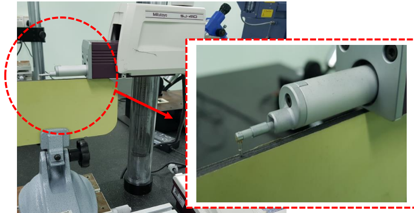
Figure 3. SJ-410 roughness tester and the display unit
