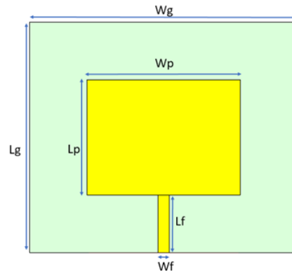
Figure 2. Parameters of patch antenna.
