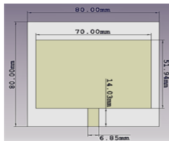
Figure 6. The structure of rectangular microstrip patch antenna added with 3 mm air gap
