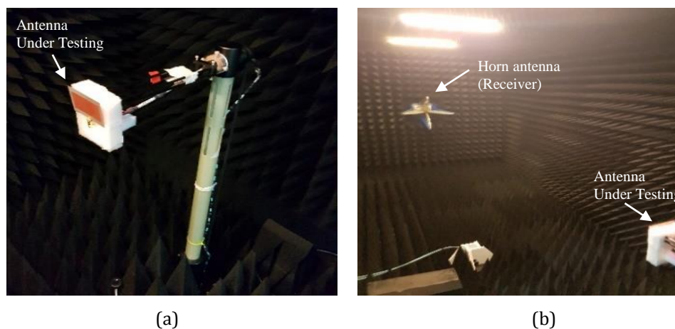
Figure 12. Radiation pattern measurement setup in anechoic chamber (a) antenna under testing (AUT) (b) AUT and receiver antenna
