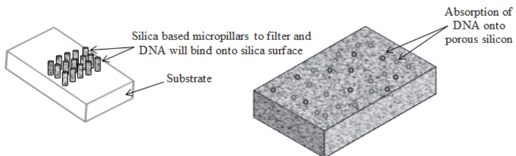
Fig. 1: Micropillars structure
