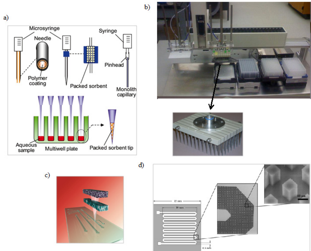
Fig. 4: Development of SPME method from in-tube to microfluidic device to extract biological compounds; a) microsyringe and micropipette in silica packed sorbent; b) auto-sampler station based on in-tip method for 96 simultaneous extractions from PAS technology, Maglada Germany; c) microfabricated device with porous silicon layer to extract and bind DNA; d) microfabricated silica pillars to filter cells based on size-exclusion and the remaining biological compound will trap into silica micropillar structure [Adapted from 12, 35, 46, 47].
