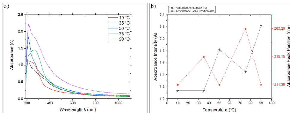
Figure 5. a) UV-Vis spectra showing the SPR absorbance of Bi NPs for water temperatures of 10, 35, 50, 75, and 90 °C. b) SPR absorbance intensity and absorbance peak position of Bi NPs as functions of water temperature.
