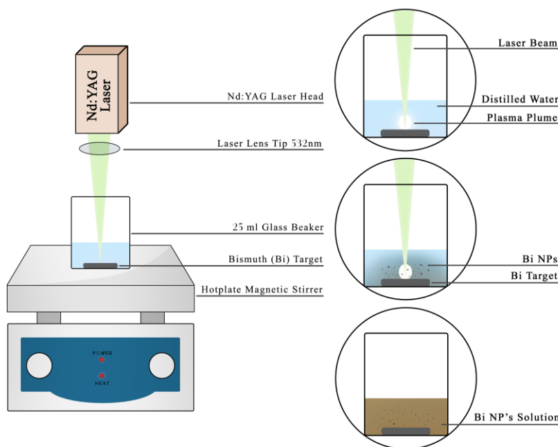
Figure 1. Schematic diagram of the experimental setup used for synthesizing the Bi NPs using PLAL.
