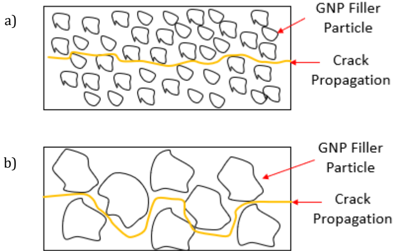
Figure 8. Drawn Crack propagation for a) 5M GNP b)15M GNP Conductive Filler
