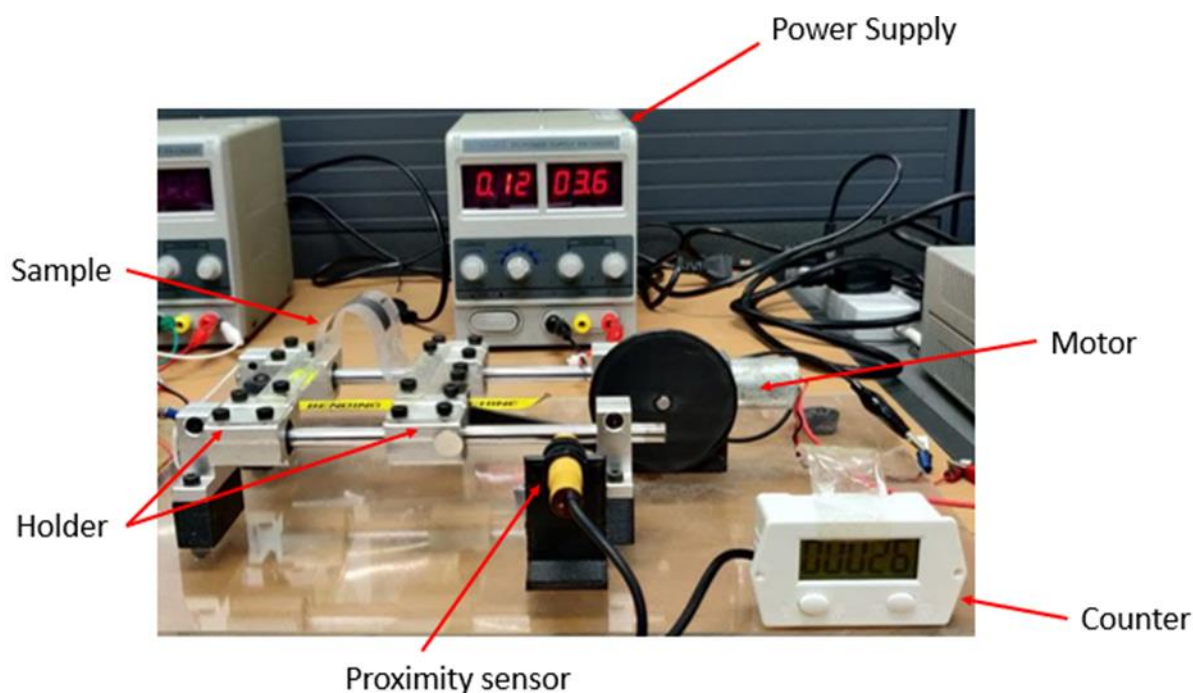
Figure 2. Cyclic Bending Test Rig Setup.
