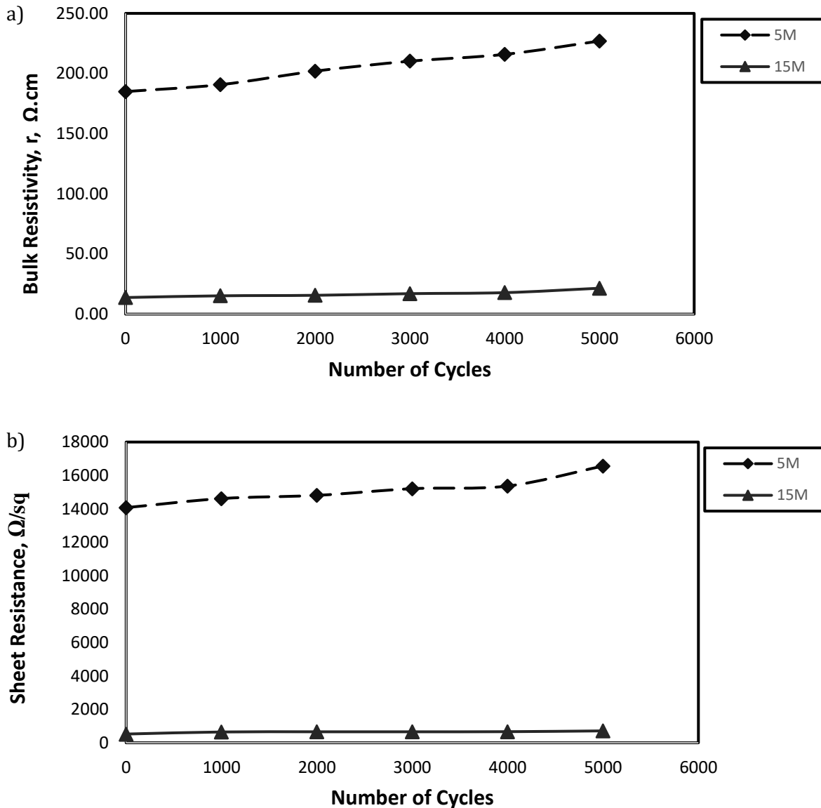
Figure 10. Graph of a) Bulk resistivity against the number of cycles b) Sheet resistivity against the number of cycles.
