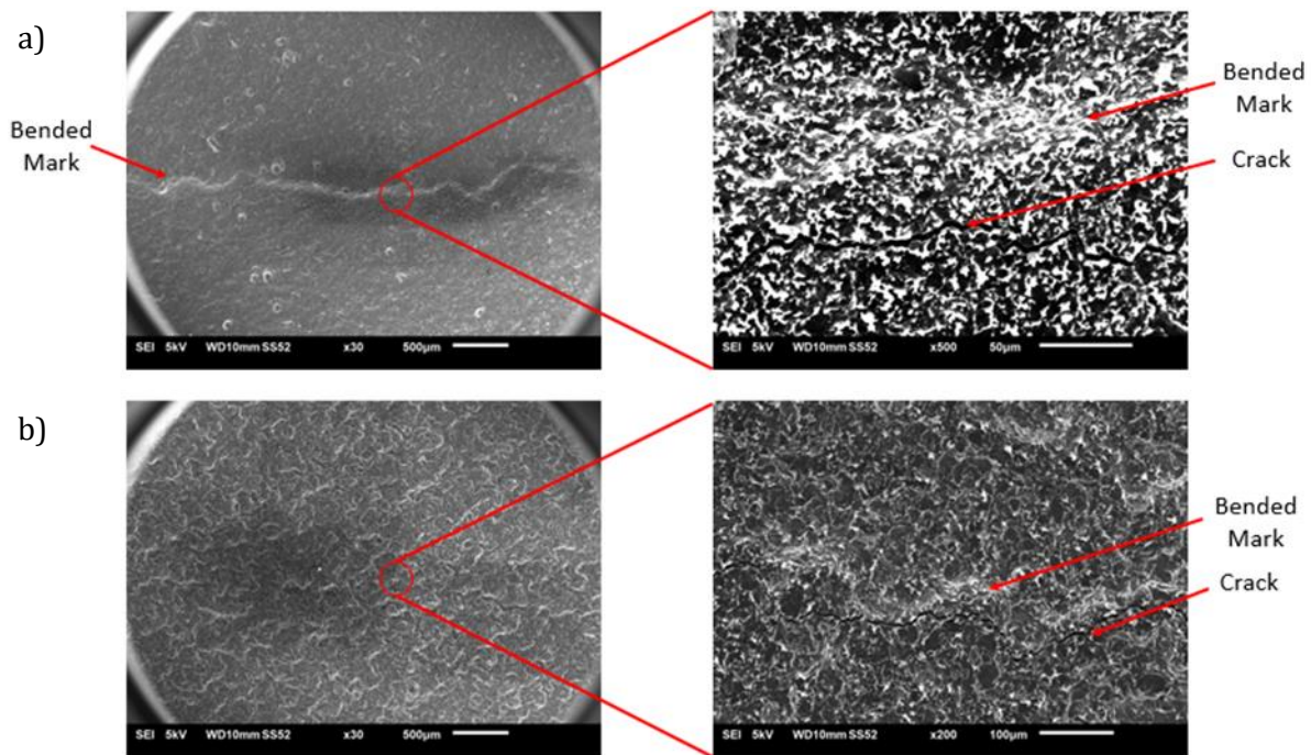
Figure 5. Morphology of a) 5M GNP conductive polymer b) 15M GNP conductive polymer after 5000 cycles of cyclic bending test.
