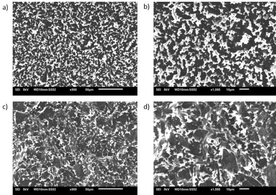
Figure 3. Surface morphology of sample a) 5M under 500 times magnification b) 5M under 1000 times magnification c) 15M under 500 times magnification d) 15M under 1000 times magnification.
