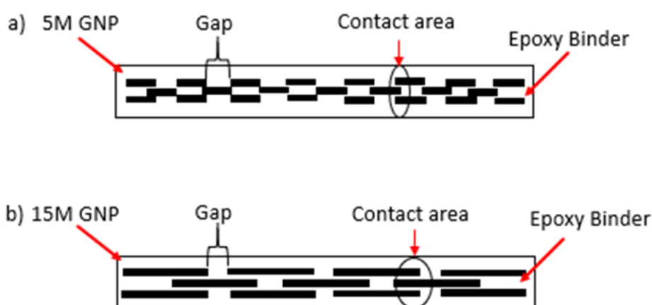
Figure 4. a) 5M GNP b) 15M GNP conductive polymer
