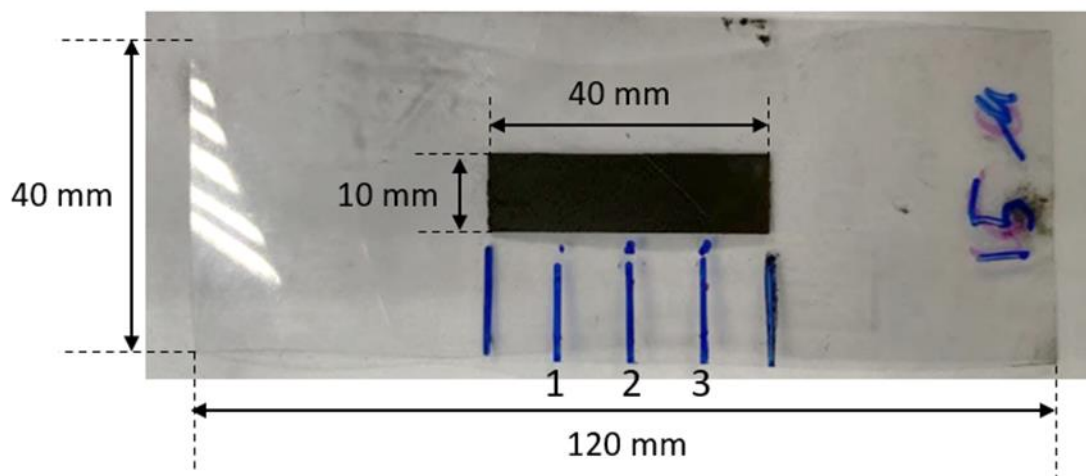
Figure 1. Sample for cyclic fatigue test (5M and 15M).
