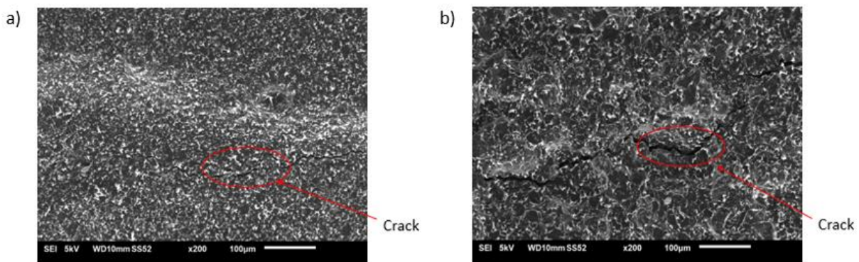
Figure 9. Crack size for a) 5M GNP b) 15M GNP conductive polymer.
