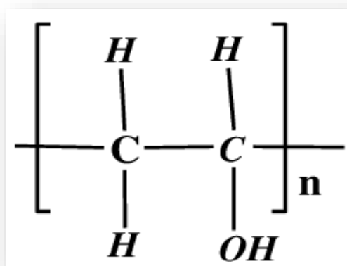
Figure1. Polyvinyl alcohol chemical structure(14).
