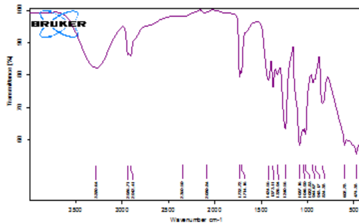
Figure (12): FTIR Spectrum for TiO 2 (15.7 nm) with weight (0.007g)/PVA Films
