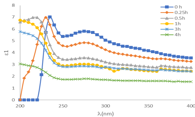
Figure 8: Correlation between the real dielectric constant and the wave-length of \text{TiO}_2/\text{PVA} films for different times of irradiation
