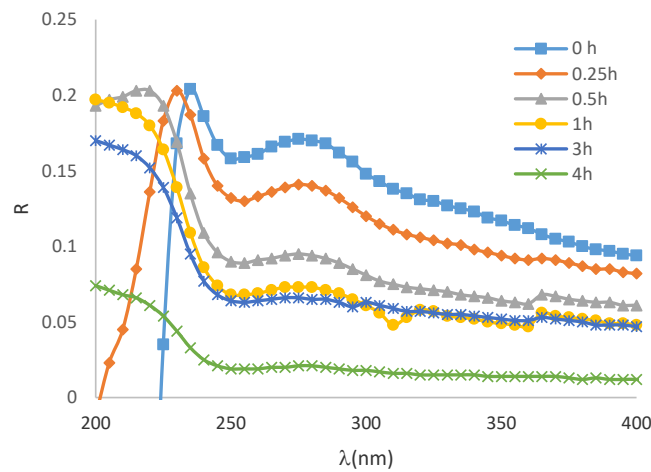
Figure 3: Reflection spectra of the TiO 2 /PVA nano-composite films for various irradiation times
