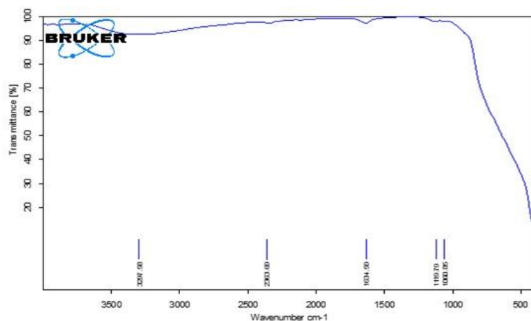
Figure 11: FTIR Spectrum for pure TiO 2 Nanoparticles Powder
