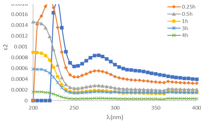
Figure 9: Correlation between the imaginary dielectric constants of the \text{TiO}_2/\text{PVA} films for different radiation times
