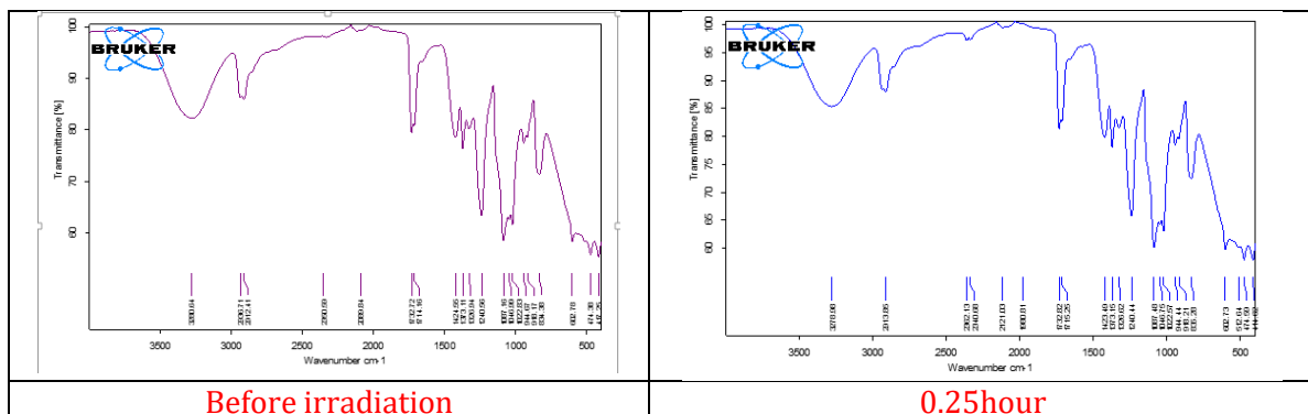
Figure (12): FTIR Spectrum for TiO 2 (15.7 nm) with weight (0.007g)/PVA Films
