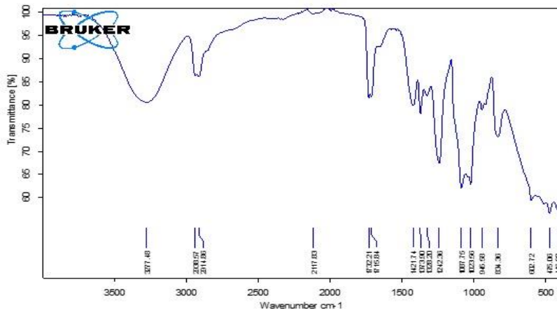
Figure 10: FTIR Spectrum for pure PVA film
