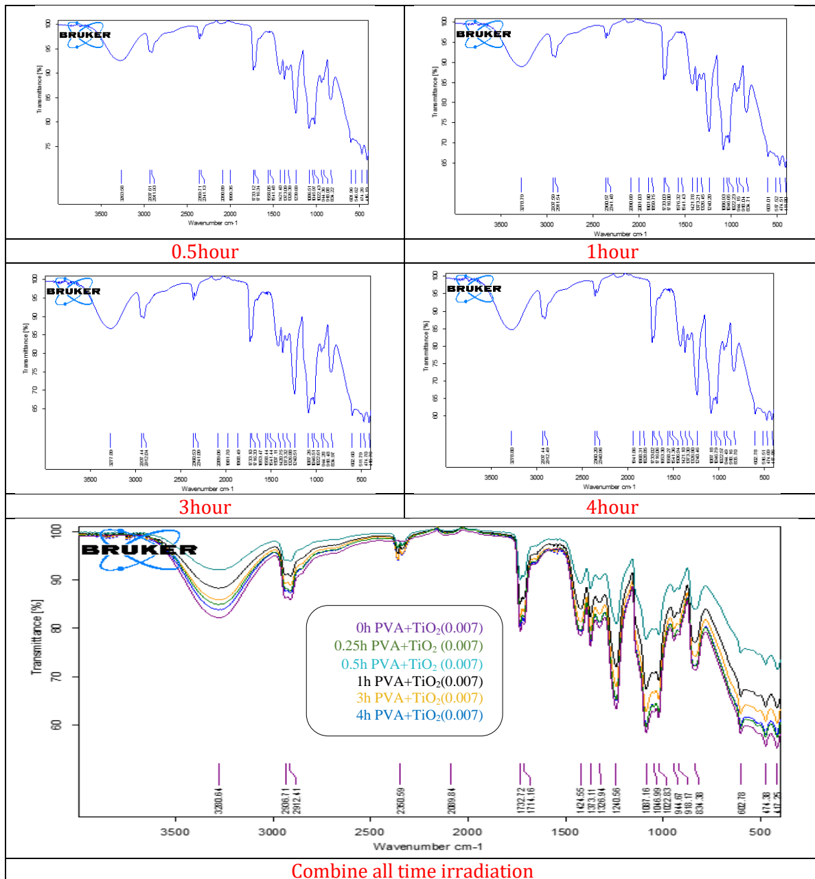
Figure (13): FT-IR spectrum for \text{TiO}_2/\text{PVA} films in various irradiation time
