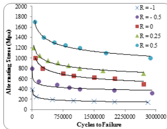
Figure 17. Influence of stress ratio on fatigue life characteristics (0% Nano)
