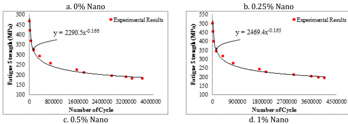
Figure 16. Curve fitting for experimental fatigue results with Nanoparticle coating and laser treatment.
