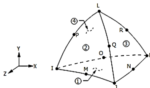
Figure 8. Element type solid 187.
