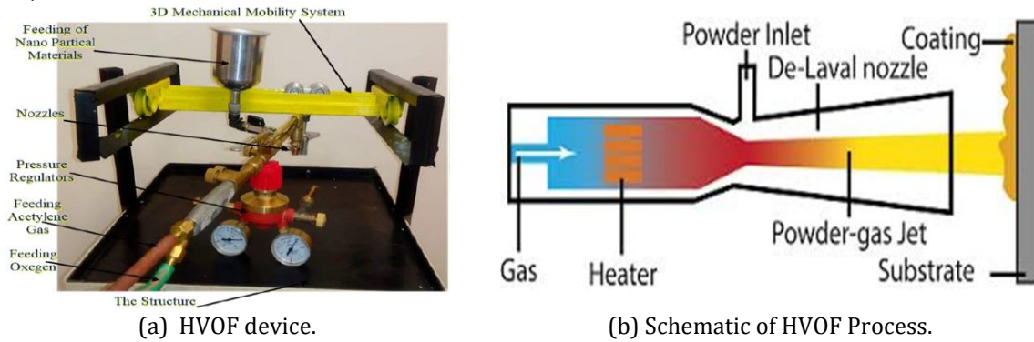
Figure 2. HVOF device and process.
