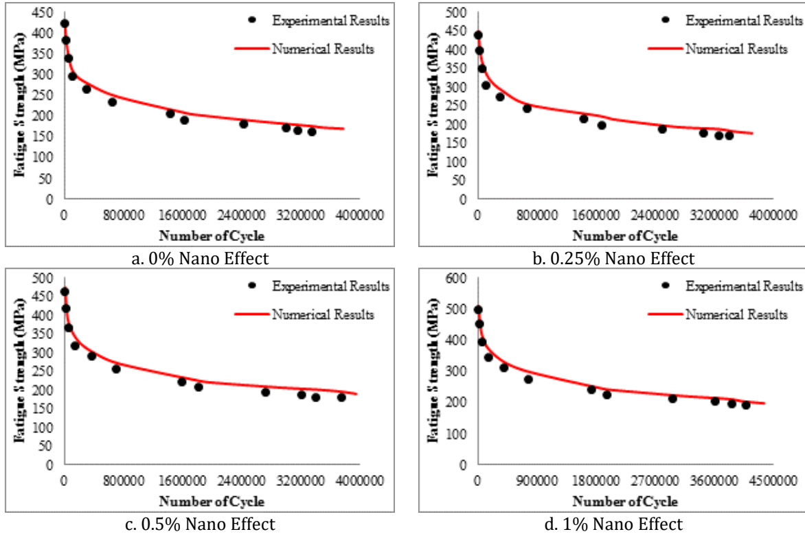
Figure 11. Numerical and experimental fatigue results comparison for steel materials with Nanomaterial and laser treatment effect.
