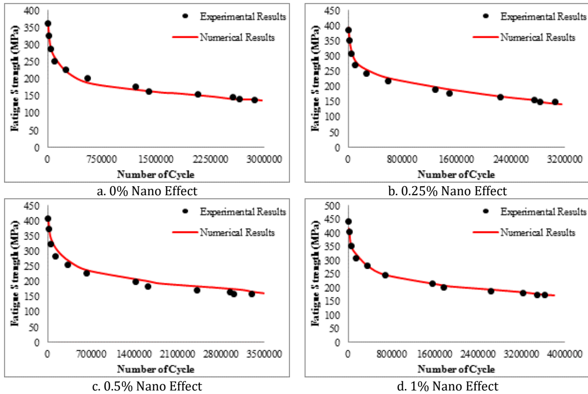
Figure 10. Numerical and experimental fatigue results comparison for steel materials with Nanomaterial.
