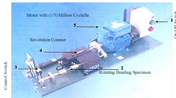
Figure 7. Bending rotating fatigue test machine
