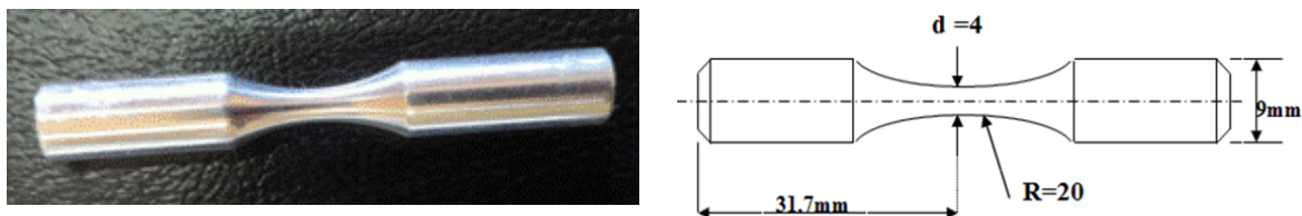
Figure 1. (a) Fatigue manufacturing sample (b) Dimensions of fatigue test specimen
