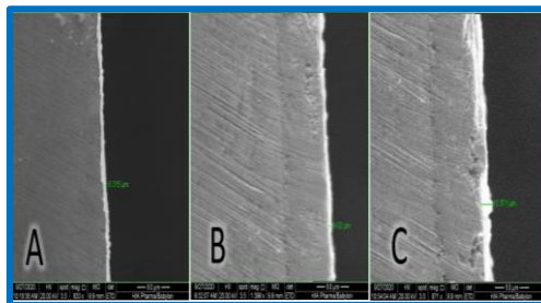
Figure 4. SEM images for coated specimens steel (a) 0.25%, (b) 0.5%, (c) 1% ZnO Nano.
