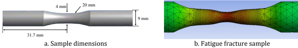
Figure 9. Fatigue sample mesh and stress distribution.
