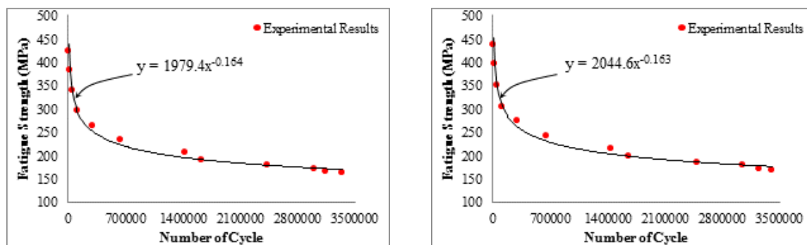
Figure 15. Curve fitting for experimental fatigue results with Nanoparticle effect, without laser treatment.
