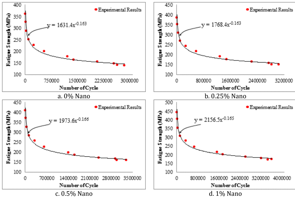
Figure 15. Curve fitting for experimental fatigue results with Nanoparticle effect, without laser treatment.
