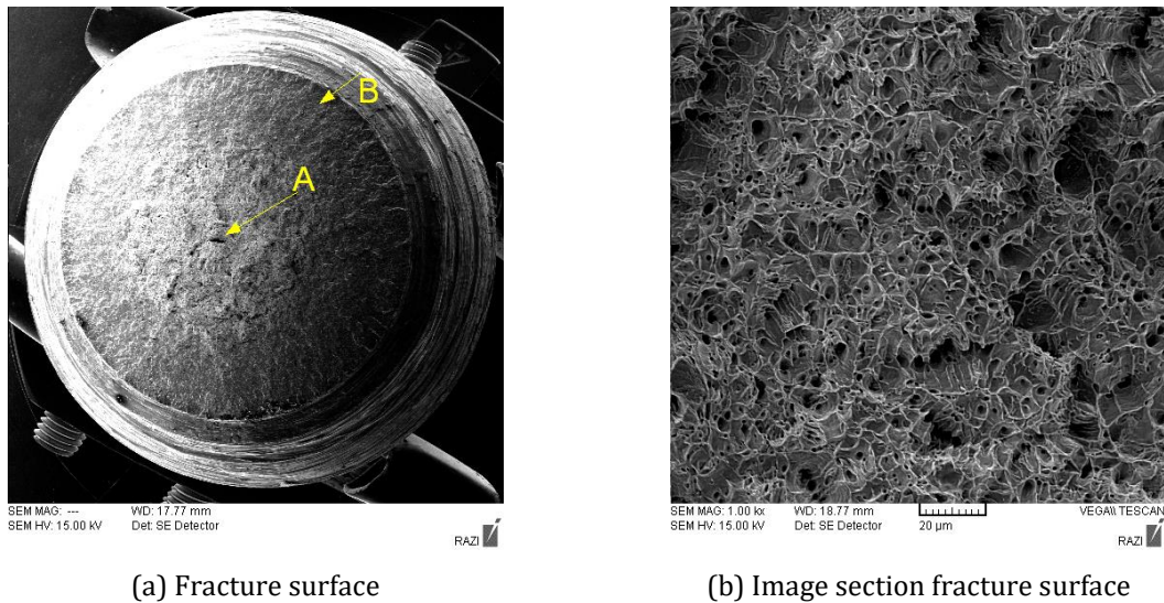
Figure 5. SEM view of the fracture surface (0% Nano) sample.
