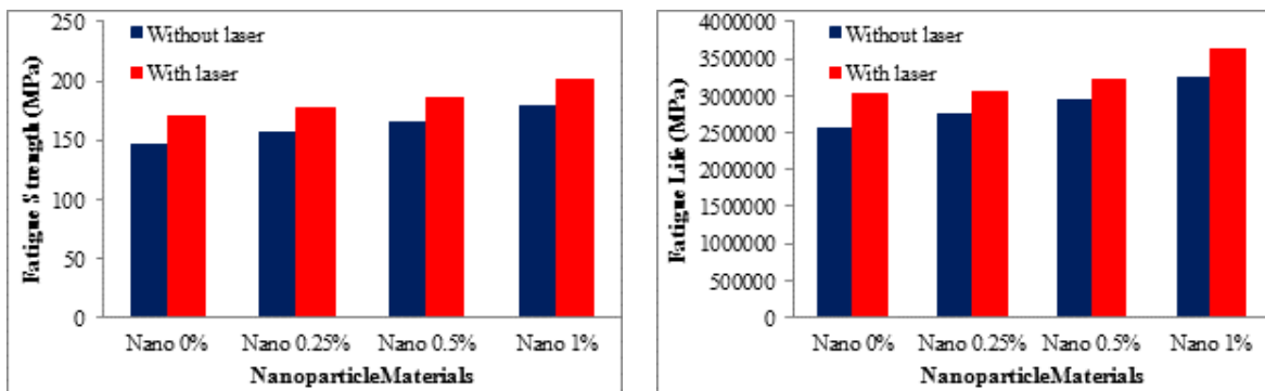
Figure 13. Fatigue characterizes material with and without laser treatment and Nano effects.
