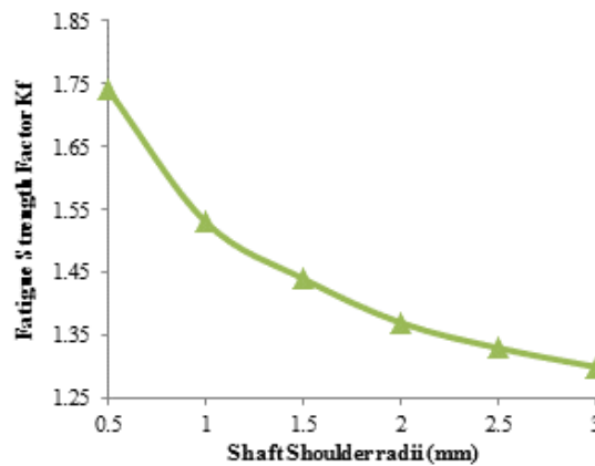
Figure 18. Fatigue strength factor for reversed bending samples (0% Nano).
