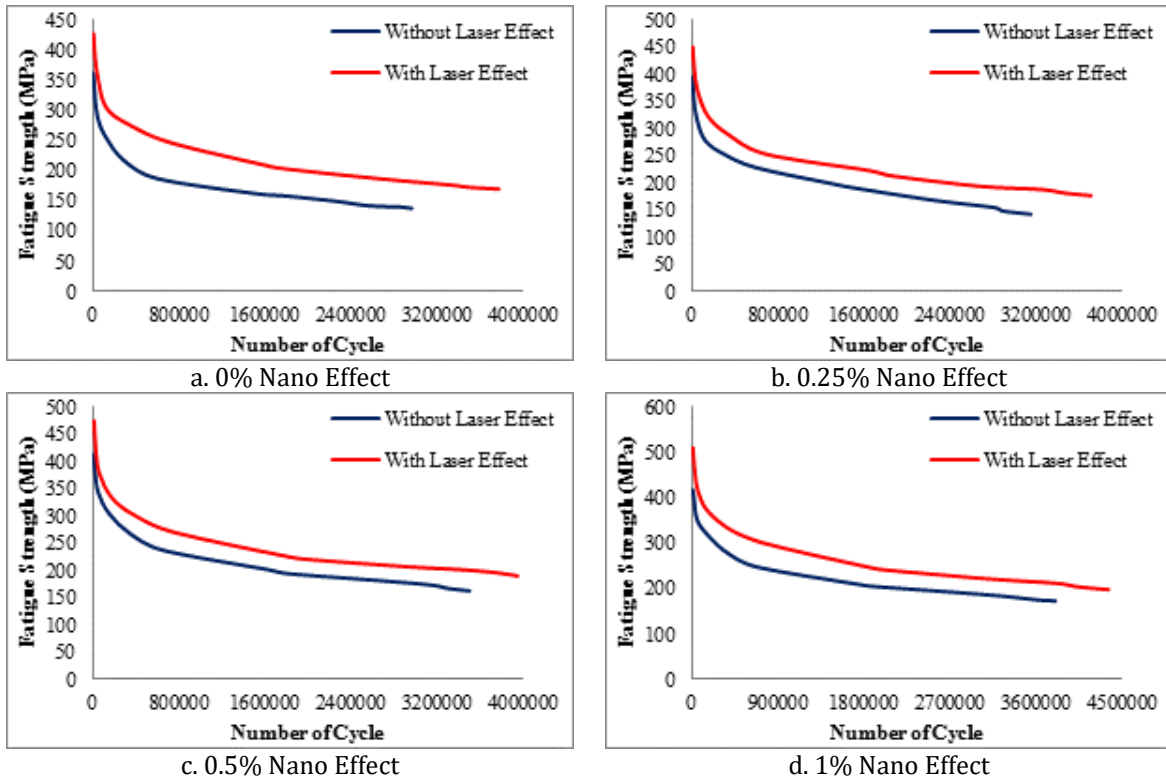
Figure 12. Results for laser treatment and Nano effect on the fatigue characterizations for materials.
