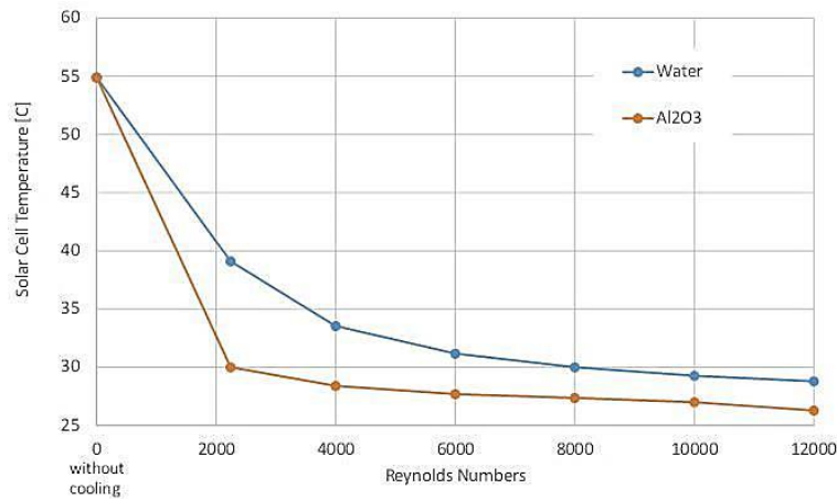
Figure 5. Photovoltaic average cell temperature as a function of Reynolds numbers.
