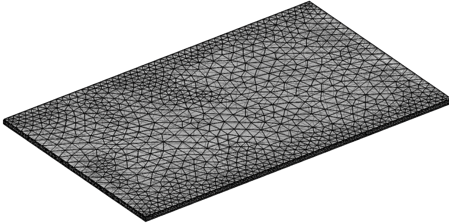
Figure 1. Computational domain and mesh of the photovoltaic cell panel.
