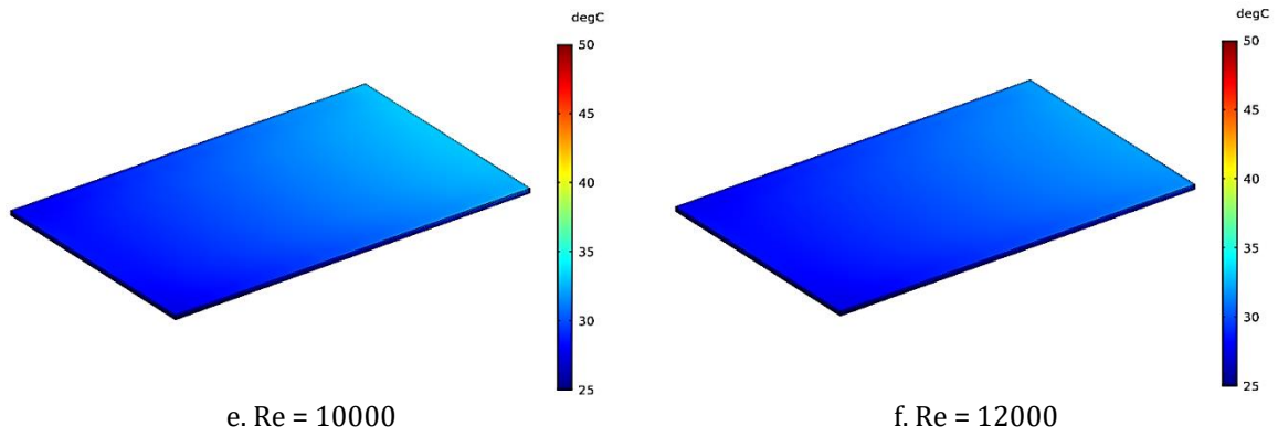
Figure 3. Temperature distribution in the photovoltaic cell structure with water cooling ( ^{\circ}\text{C} ) for a range of Reynolds numbers.
