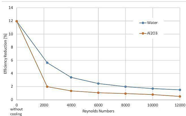
Figure 6. Photovoltaic electrical efficiency reduction as a function of Reynolds numbers.
