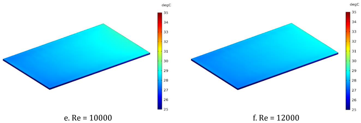
Figure 4. Temperature distribution in the photovoltaic cell structure with nanofluid Al 2 O 3 cooling (°C) for a range of Reynolds numbers.
